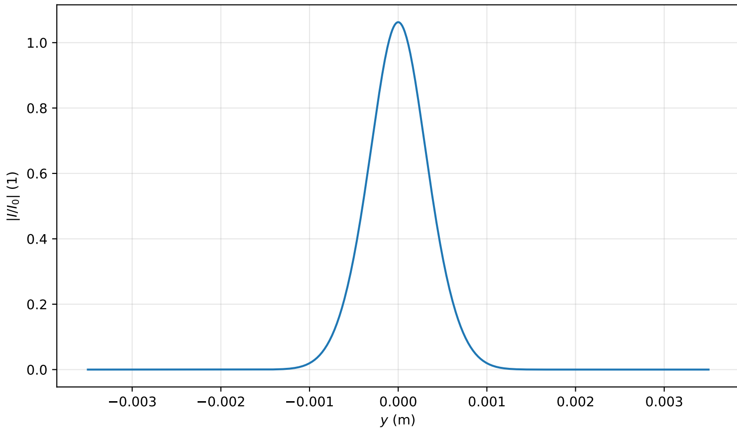
Intensity profile I(x=0, y, z=0.478)/I_0 , P_{in}=0.6P_{cr} , artificial time
